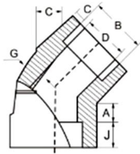
SW 45° Elbow
