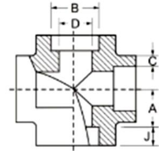
SW Cross
