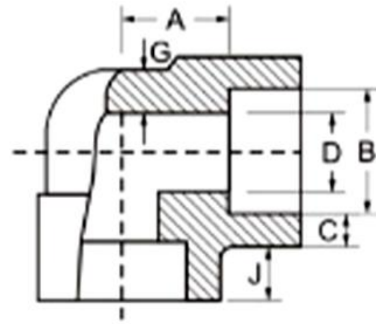
SW 90° Elbow
